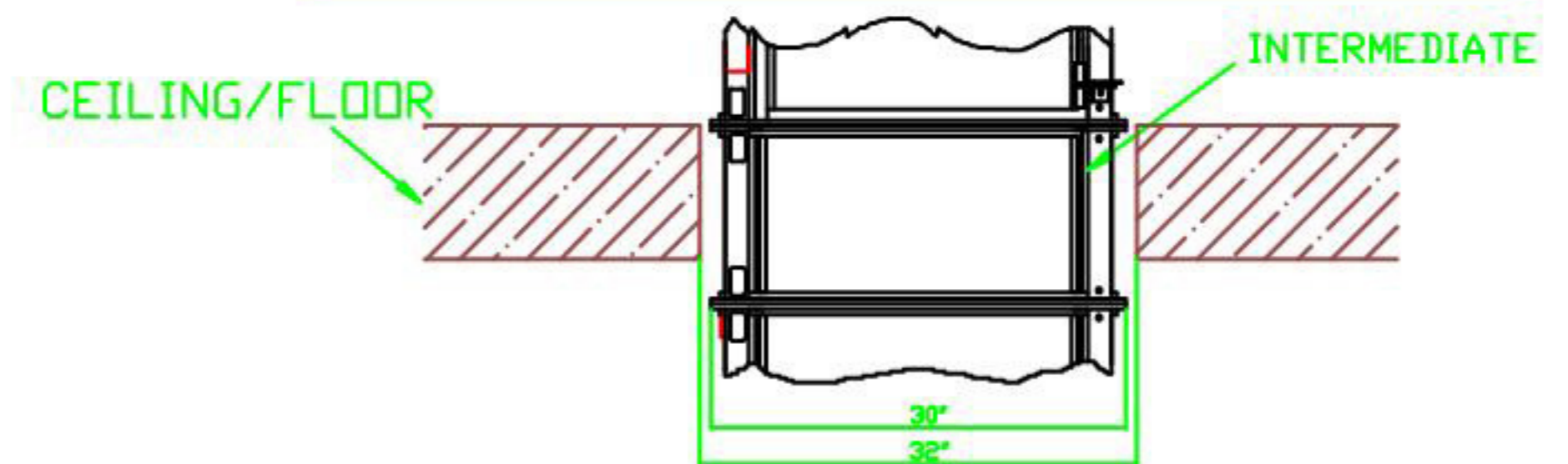
DETAIL "A" (TYPICAL OF FLOOR PENETRATION)
