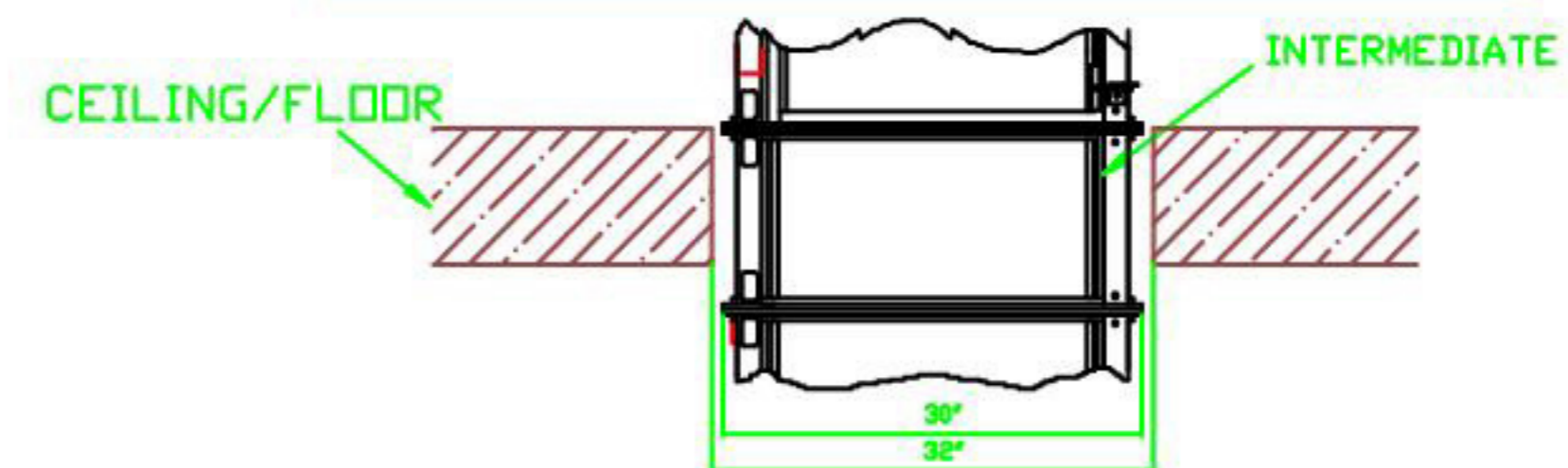
DETAIL "A" (TYPICAL OF FLOOR PENETRATION)
